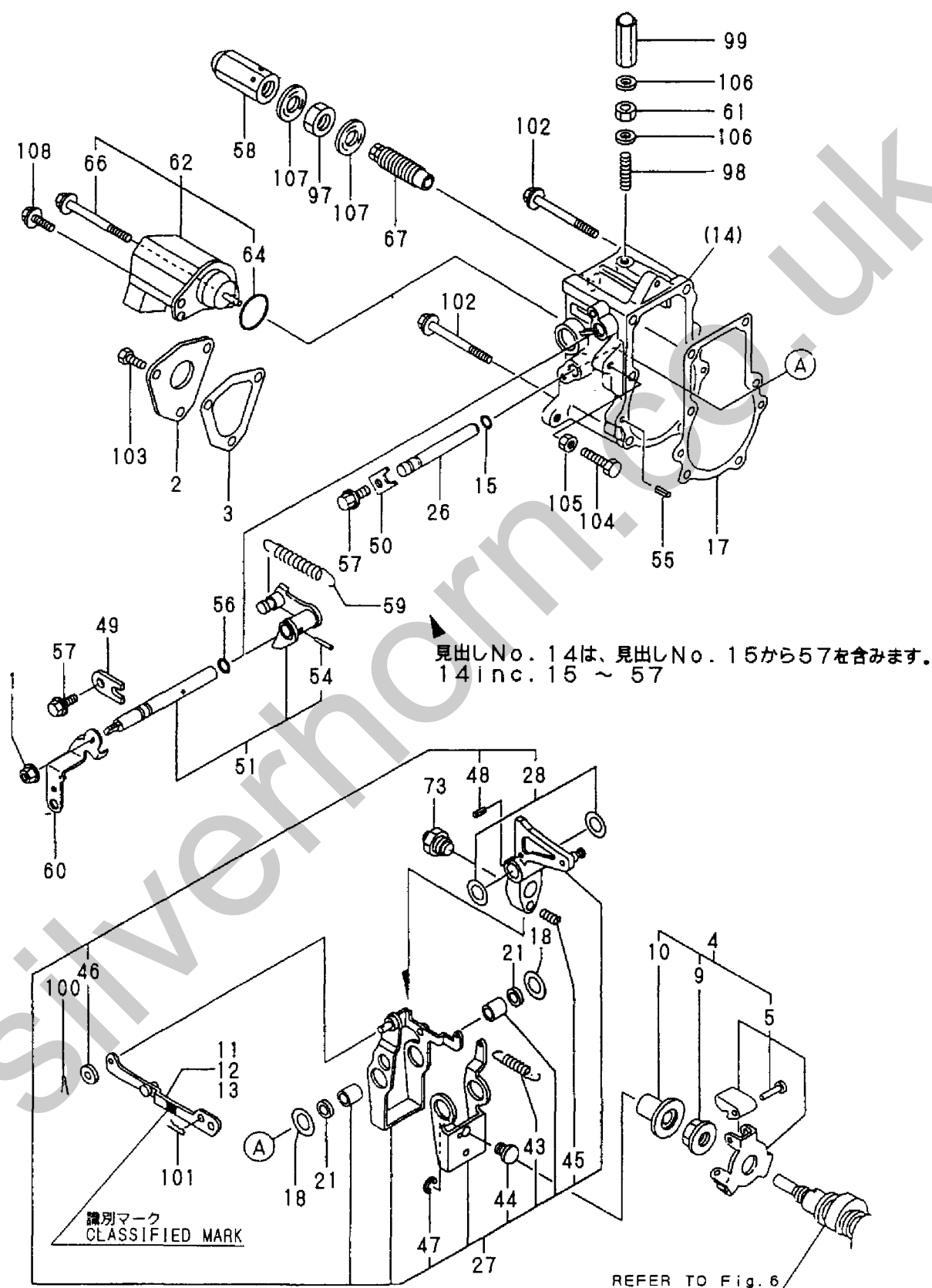
Fig. 11 ガバナ GOVERNOR
